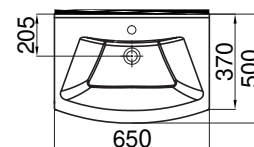
2801-0655 Vega Lavabo (50x65) Vega Furniture Washbasin
