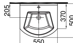
2801-0555 Vega Lavabo (50x55) Vega Furniture Washbasin
