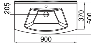
2801-0905 Vega Lavabo (50x90) Vega Furniture Washbasin
